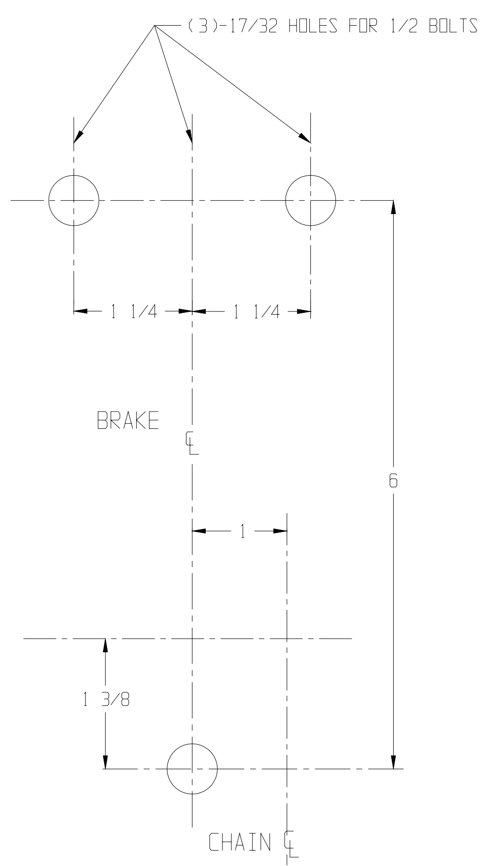
DRILLING DIAGRAM
