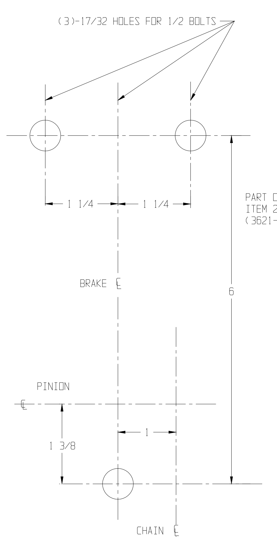
DRILLING DIAGRAM
